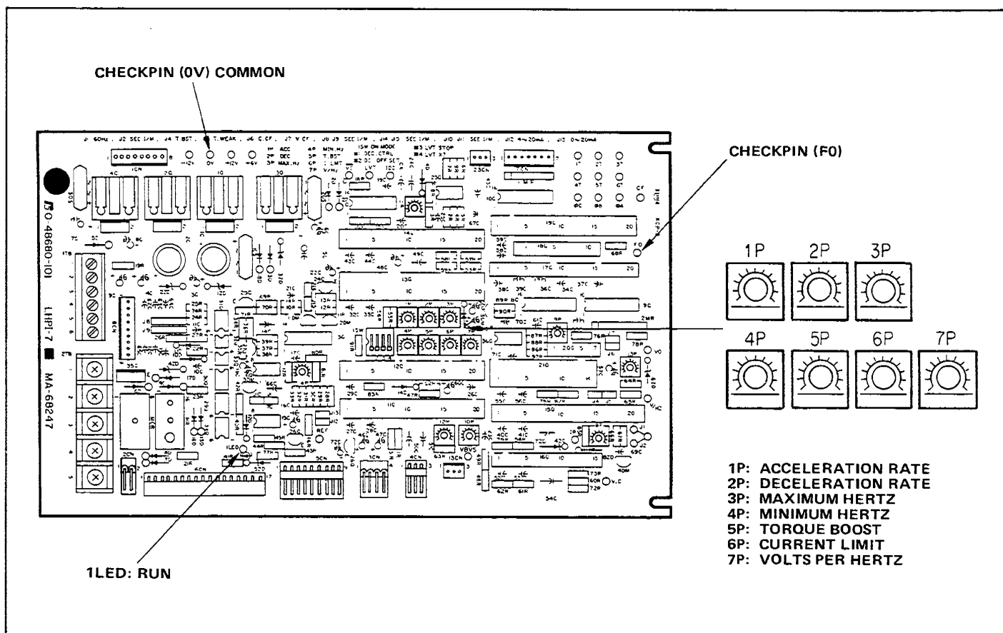
Figure 4-1. Regulator Pots, LED and Checkpins.
