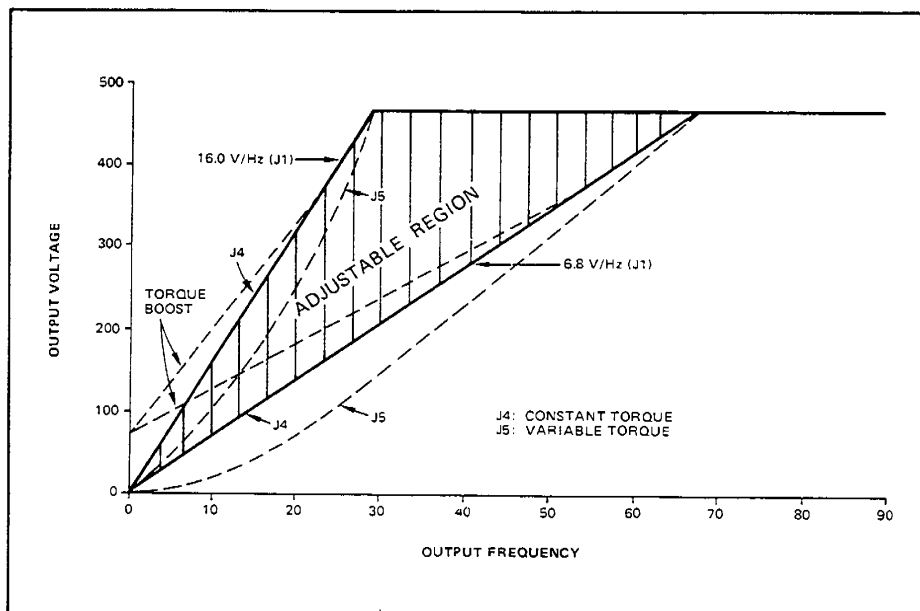
Figure 4-2. Volts/Hertz Pot Adjustable Region for 460 V Input.
