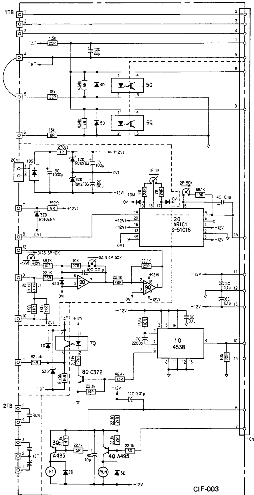
Figure 6-11. Typical Customer Interface PC Board Schematic.
