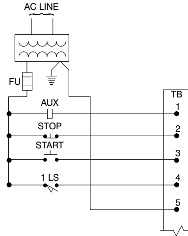
61C501 Typical Field Signal Connections
