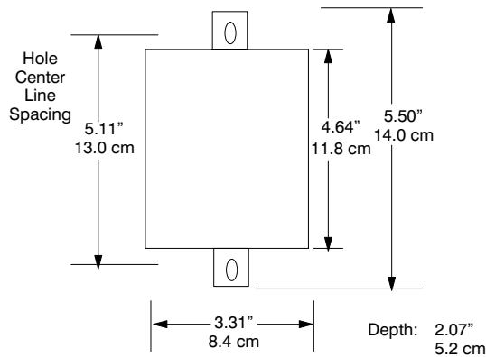
M/N 61C545 Panel-Mount Terminal Board
