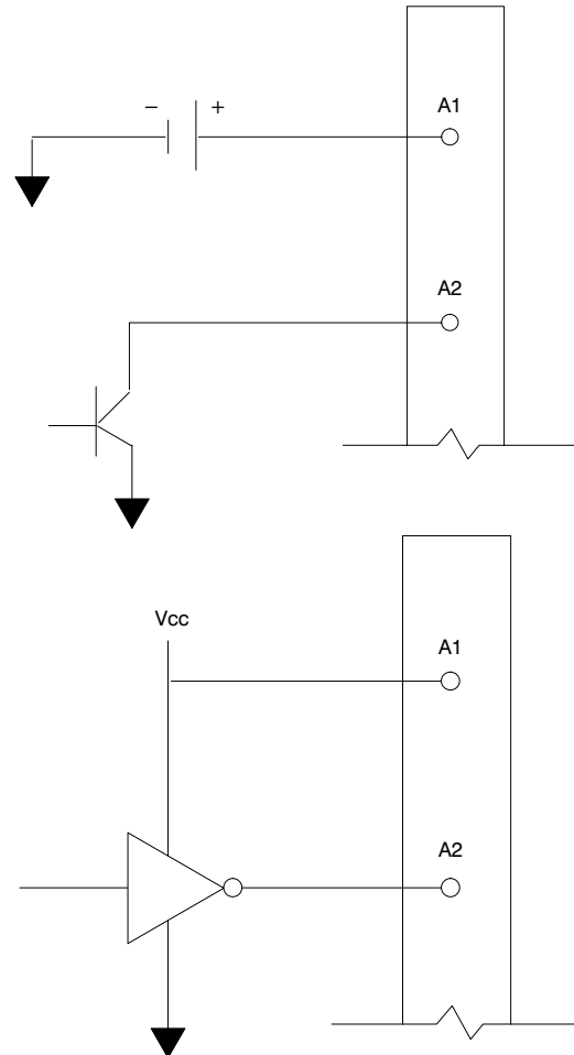
57C419 Typical Field Connections for Open Collector TTL
