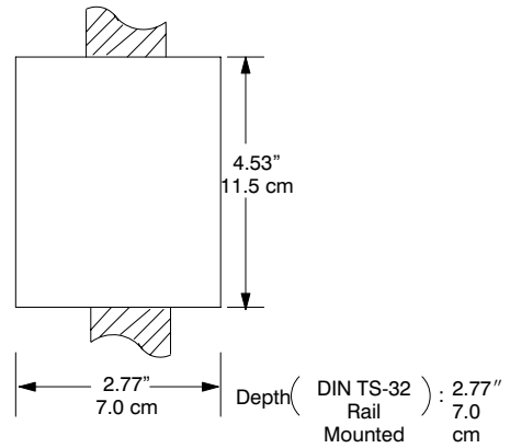
M/N 61C546 DIN Rail-Mount Terminal Board
