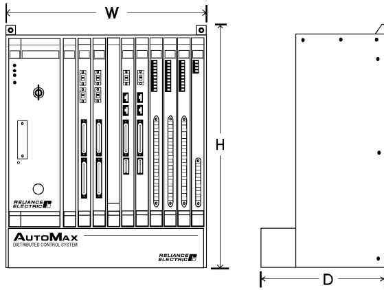
6, 10 and 16 Card Racks
