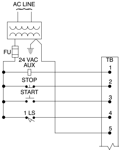
61C516 Typical Field Signal Connections
