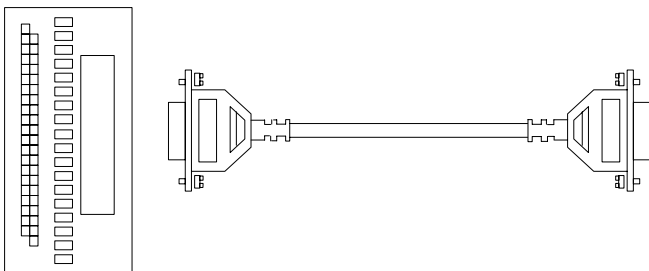
M/N 61C549 Terminal Board and Cable Assembly (M/N 61C550 is similar)
