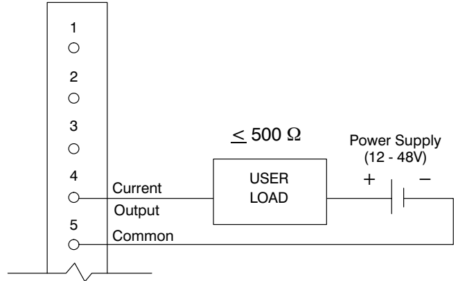
57C410 Typical Field Connections for 4-20 mA Current Output
