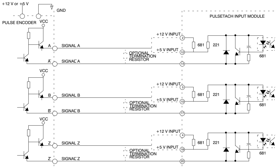
57C421 Typical Pulsetach Connections for a 5V dc Differential Input
