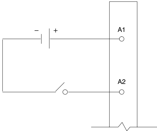
57C419 Typical Field Connection for Contact Closures
